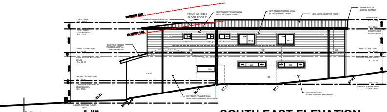
SOUTH EAST ELEVATION
